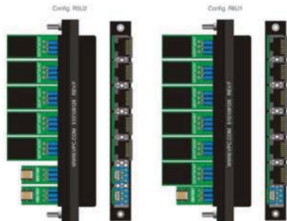
J90RJ45T 7200.98 RJ45 (Ethernet 100 Base T) to 90 Series interface
